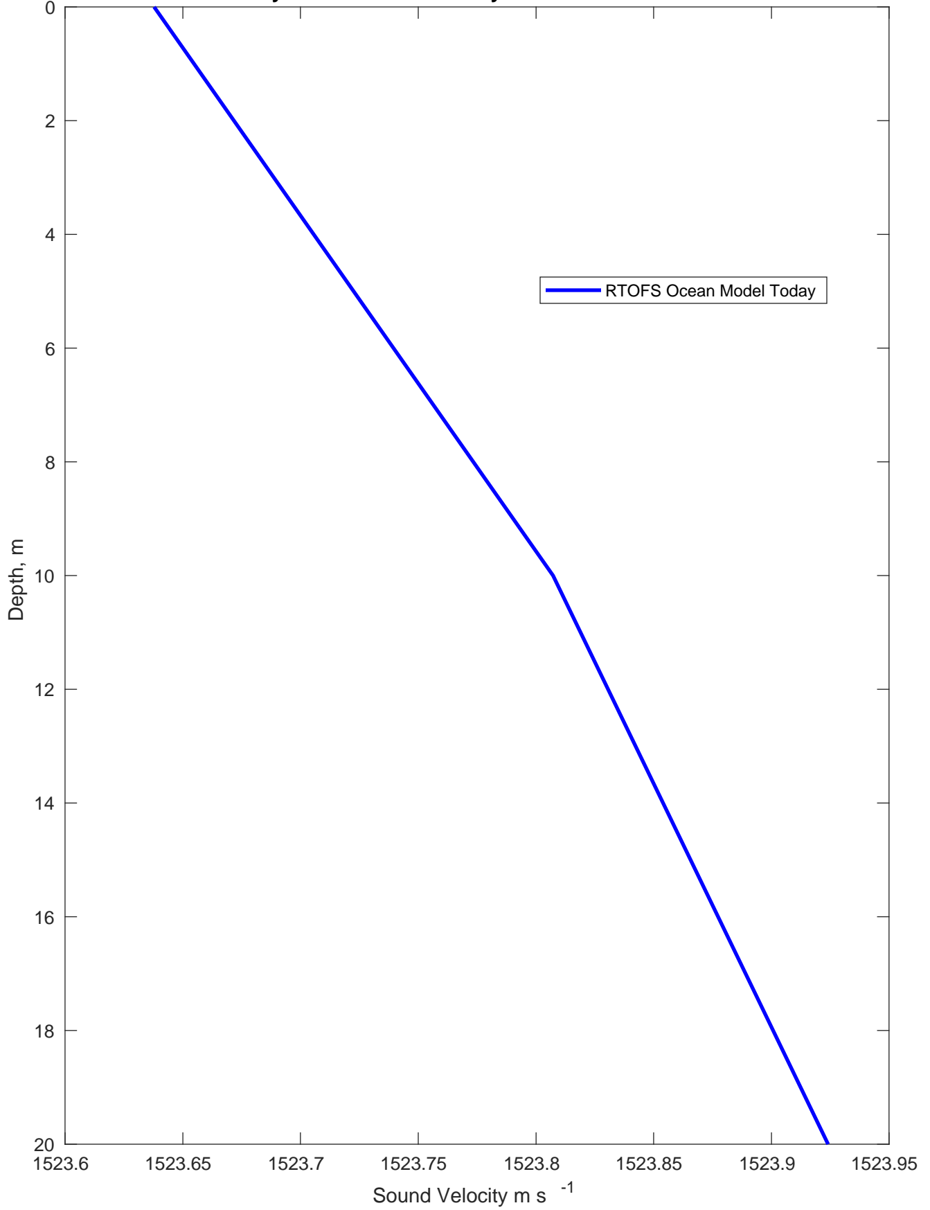
Sound Velocity Profile for TABS Buoy J on 08-Dec-2020 00:00:00
